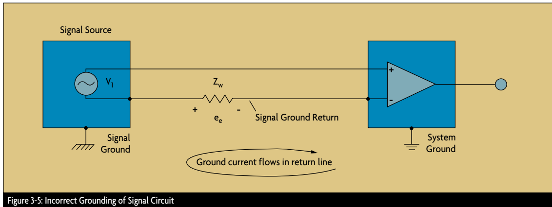
Figure 3-5: Incorrect Grounding of Signal Circuit
