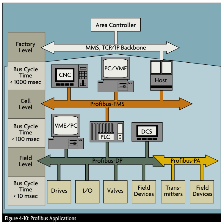
Figure 4-10: Profibus Applications
